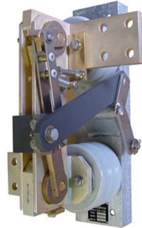
1200 AMP 1000 VDC REMOTE HANDLE OPERATED DISCONNECT FOR POLE MOUNTING
